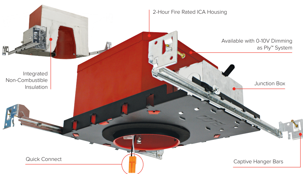
4" and 6" Shallow New Construction Housings
