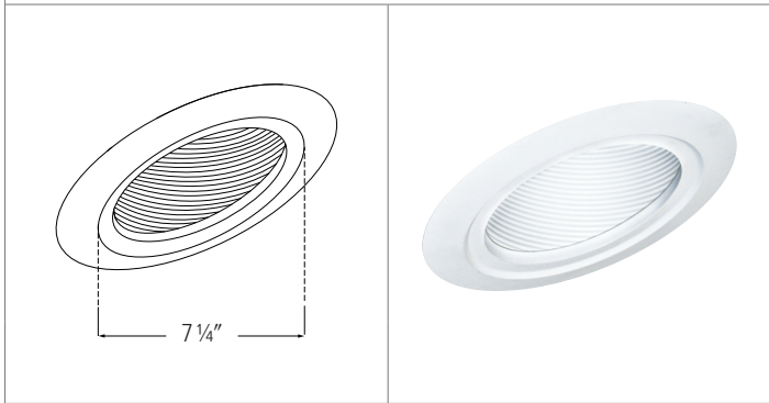
EL560 - 5" BAFFLE WITH ADJUSTABLE GIMBAL RING
