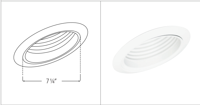
ELM531K - 5" ADJUSTABLE BAFFLE WITH SOCKET BRACKET
