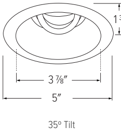
ELK4717 - 4" ROUND ADJUSTABLE DEEP REFLECTOR
