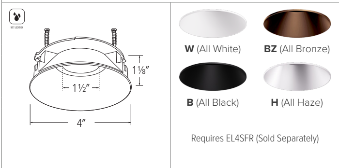
ELK408 - 4" ROUND TRIMLESS REFLECTOR
