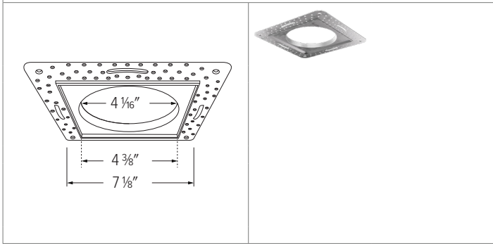
EL4FMS - 4" SQUARE FLUSH MOUNT SPACKLE FRAME
