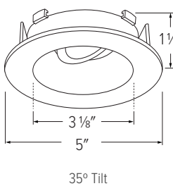
ELK4721 - 4" ROUND ADJUSTABLE REFLECTOR
