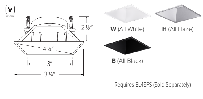
ELK445 - 4" SQUARE TRIMLESS REFLECTOR
