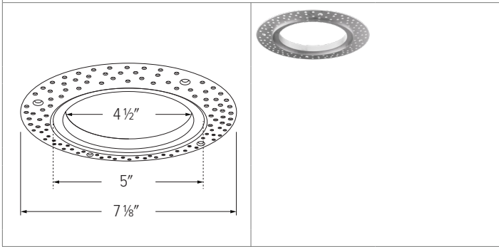
EL4FMR - 4" ROUND FLUSH MOUNT TRIM ADAPTER
