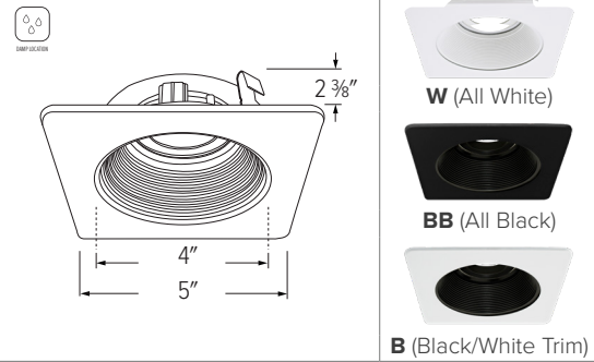
ELK4293 - 4" SQUARE PHENOLIC BAFFLE
