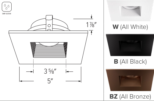
ELK4284 - 4" SQUARE ADJUSTABLE BAFFLE
