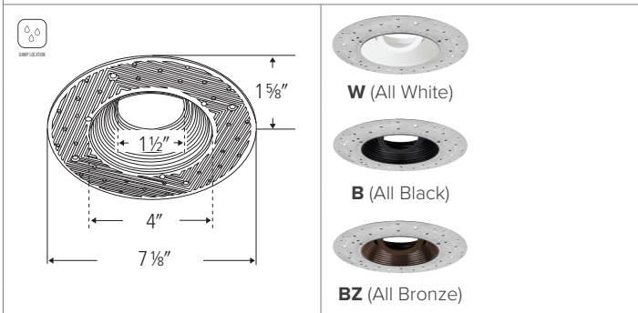
ELK434 - 4" ROUND TRIMLESS ADJUSTABLE BAFFLE
