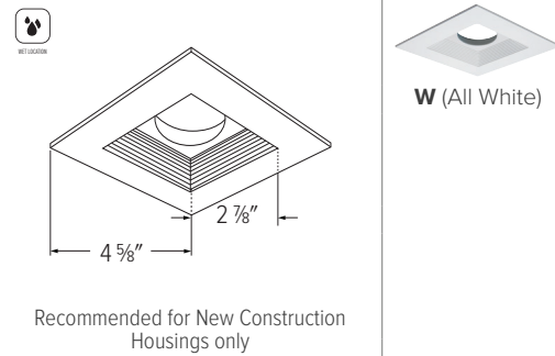
ELK4716 - 4" SQUARE BAFFLE
