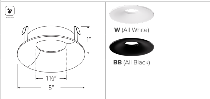
ELK4172 - 4" ROUND CURVED REFLECTOR
