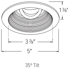
ELK4719 - 4" ROUND DEEP BAFFLE
