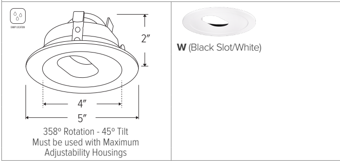
ELK4120 - 4" ROUND ROTATABLE SLOT APERTURE
