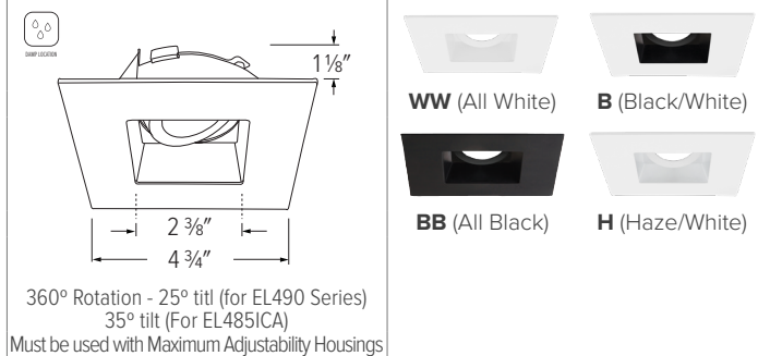
ELK4759 - 4" SQUARE ADJUSTABLE REFLECTOR
