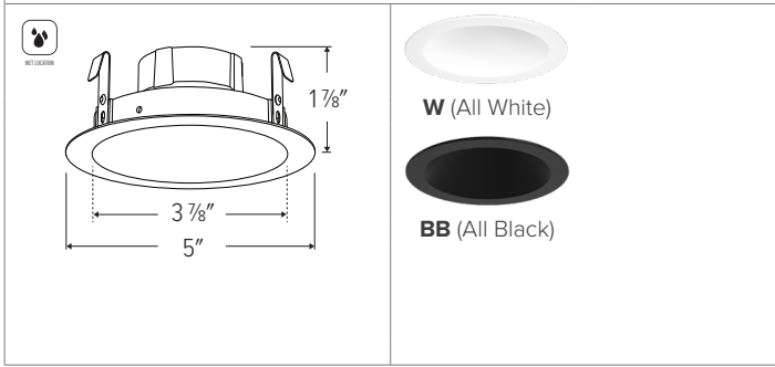
ELK4163 - 4" ROUND MICRO FLANGE REFLECTOR
