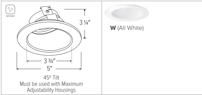
ELK4122 - 4" ROUND ADJUSTABLE REFLECTOR WALL WASH
