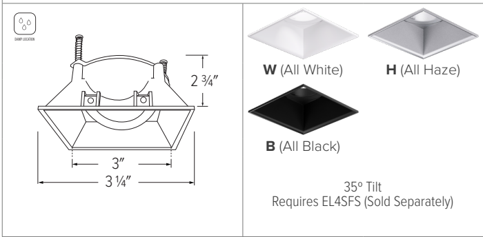
ELK459 - 4" SQUARE ADJUSTABLE TRIMLESS REFLECTOR
