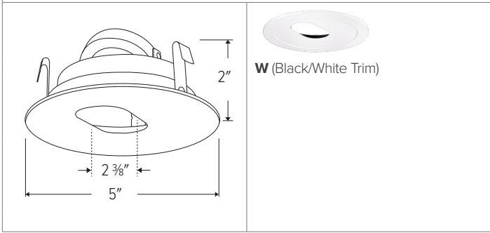
ELK4130 - 4" ROUND SLOT APERTURE
