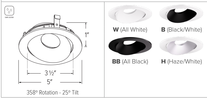
ELK4179 - 4" ROUND DIRECTIONAL GIMBAL
