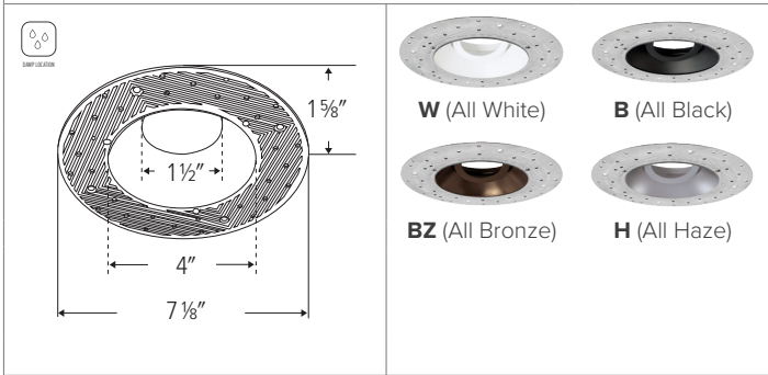
ELK430 - 4" ROUND TRIMLESS ADJUSTABLE SMOOTH REFLECTOR
