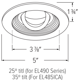
ELK4713 - 4" ROUND ADJUSTABLE BAFFLE
