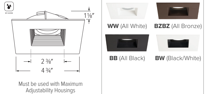
ELK4743 - 4" SQUARE BAFFLE
