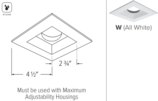
ELK4714 - 4" SQUARE REFLECTOR
