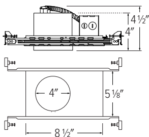
EJB4ICA NEW CONSTRUCTION HOUSING FOR 2-HOUR FIRE RATED CEILINGS
