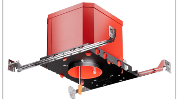
EL48FICA 2-HOUR FIRE RATED NEW CONSTRUCTION HOUSING
