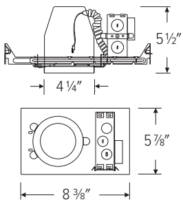
EL490ICA STANDARD NEW CONSTRUCTION HOUSING
