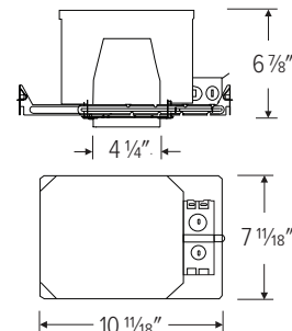
EL48FICA 2-HOUR FIRE RATED NEW CONSTRUCTION HOUSING
