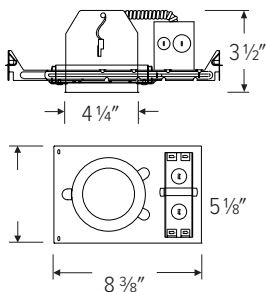
EL492ICA SHALLOW NEW CONSTRUCTION HOUSING
