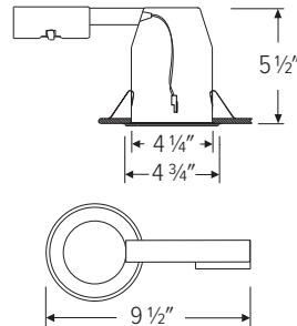
EL490RICA STANDARD REMODEL HOUSING
