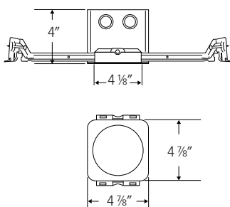
EJB483ICA NEW CONSTRUCTION HOUSING JUNCTION BOX FOR 2-HOUR FIRE RATED CEILINGS
