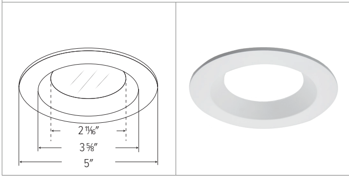
ELL4812 DIECAST LENSED REFLECTOR TRIM
