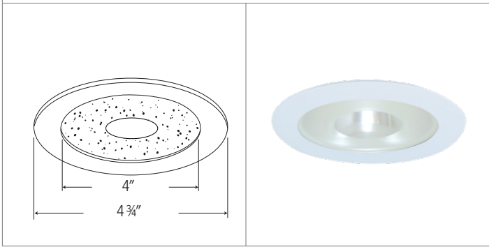
EL9115 SHOWER TRIM WITH FROSTED PINHOLE GLASS
