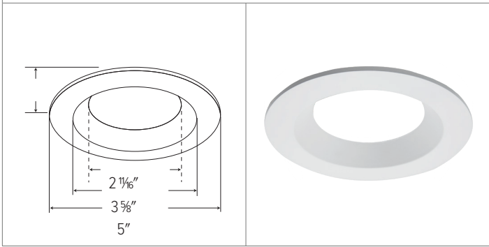
ELL4810 DIECAST REFLECTOR TRIM
