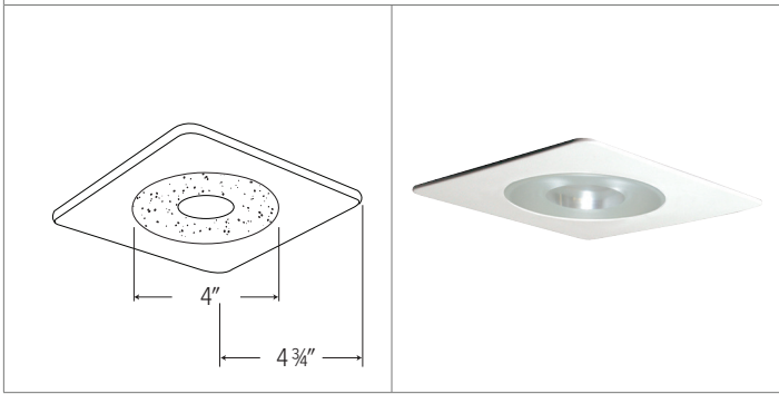
EL2915 SHOWER TRIM WITH FROSTED PINHOLE GLASS
