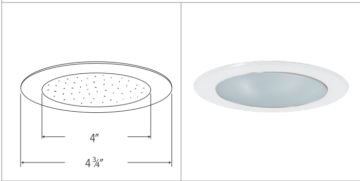
EL9112 OPEN TRIM
