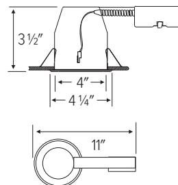
EL492RICA IC AIRTIGHT SHALLOW REMODEL DEDICATED LED HOUSING
