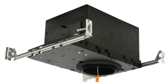
EL490AJICA/EL490AJICA-EM7 - DEDICATED LED IC AIRTIGHT NEW CONSTRUCTION R60 AND CHICAGO PLENUM HOUSING
