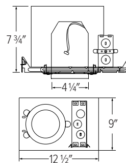
EL49FICA-GU10 2-HOUR FIRE RATED NEW CONSTRUCTION HOUSING
