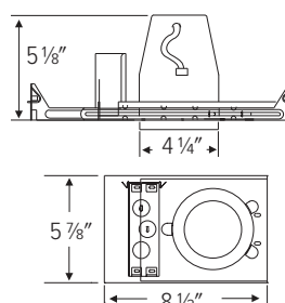
EL49LDICA/EL49LDICA-7 NEW CONSTRUCTION IC AIRTIGHT HOUSING
