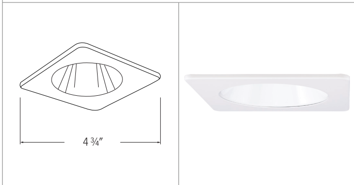
EL2421 - 4" SQUARE SPECULAR REFLECTOR
