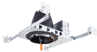
EL490ICA/EL490ICA-7/ EL490ICA-EM5 NEW CONSTRUCTION IC AIRTIGHT HOUSING
