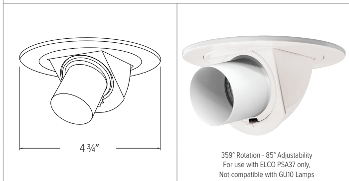
EL1487 - 4" ADJUSTABLE PULL DOWN WITH DIRECTIONAL SNOOT
