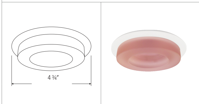
EL1452 - 4" FROSTED GLASS
