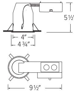
EL490RICA/EL490RICA-EM5 REMODEL DEDICATED LED IC AIRTIGHT HOUSING
