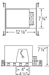
EL49ICA DOUBLE WALL NEW CONSTRUCTION IC HOUSING FOR GU10 BASE
