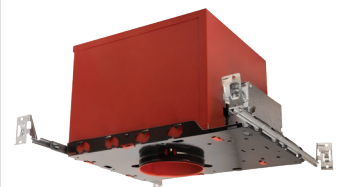
EL49FICA-GU10 2-HOUR FIRE RATED NEW CONSTRUCTION HOUSING
