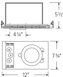
EL490AJICA/EL490AJICA-EM7 - DEDICATED LED IC AIRTIGHT NEW CONSTRUCTION R60 AND CHICAGO PLENUM HOUSING
