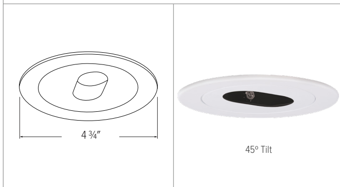
EL1420 - 4" ADJUSTABLE SLOT SPINNABLE APERTURE
