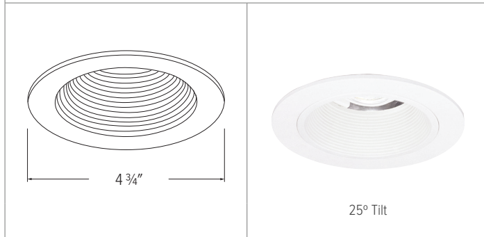
EL1493D - 4" ADJUSTABLE PHENOLIC STEP BAFFLE WITH DIECAST TRIM RING
