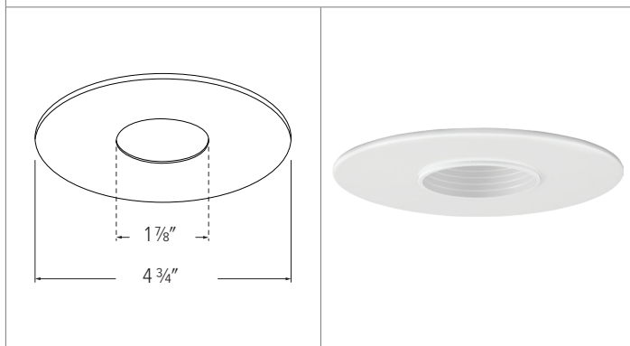
EL1419 - 4" PINHOLE APERTURE WITH BAFFLE
