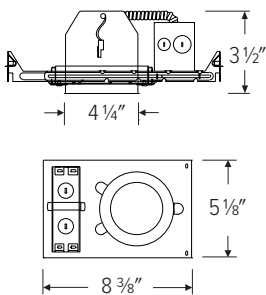
EL492ICA/EL492ICA-7 IC AIRTIGHT SHALLOW NEW CONSTRUCTION HOUSING
