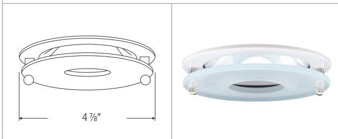
EL1426 - 4" CHROME REFLECTOR WITH SUSPENDED FROSTED GLASS
