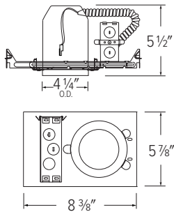
EL490ICA/EL490ICA-7/ EL490ICA-EM5 NEW CONSTRUCTION IC AIRTIGHT HOUSING
