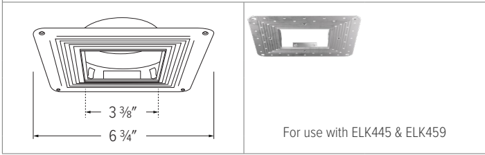
EL4SFS - 4" SQUARE TRIMLESS SPACKLE FRAME
