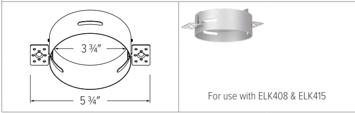
EL4WCARD - 4" ROUND TRIMLESS WOOD CEILING RING
