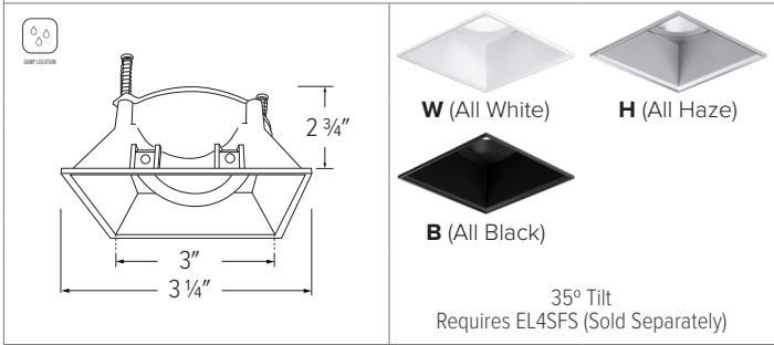
ELK459 - 4" SQUARE ADJUSTABLE TRIMLESS REFLECTOR
