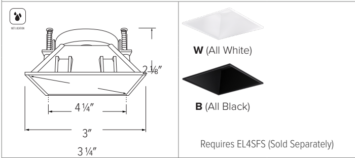
ELK445 - 4" SQUARE TRIMLESS REFLECTOR
