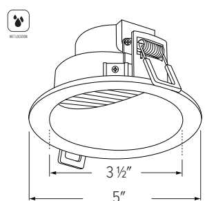
EKCL4183 - 4" ROUND SLEEK LENSED WALL WASH REFLECTOR
