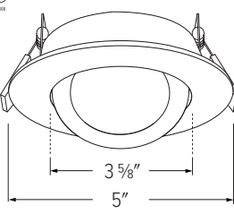
EKCL4188 - 4" ROUND ADJUSTABLE SPOT
