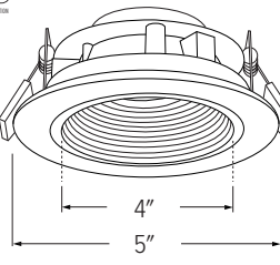
EKCL4193 - 4" ROUND ADJUSTABLE BAFFLE
