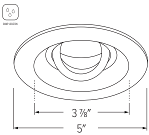
EKCL4710 - 4" ROUND ADJUSTABLE REFLECTOR
