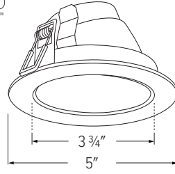
EKCL4122 - 4" ROUND ADJUSTABLE REFLECTOR WALL WASH
