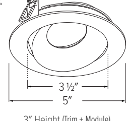
EKCL4179 - 4" ROUND DIRECTIONAL GIMBAL
