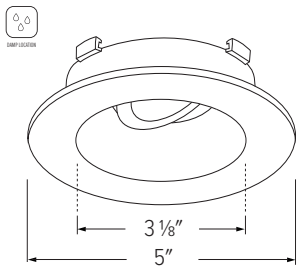
EKCL4721 - 4" ROUND REFLECTOR
