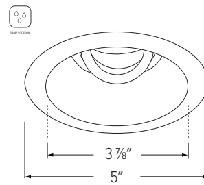
EKCL4717 - 4" ROUND ADJUSTABLE DEEP REFLECTOR
