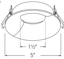
EKCL4172 - 4" ROUND CURVED REFLECTOR
