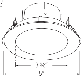
EKCL4118 - 4" ROUND DEEP REFLECTOR
