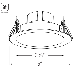
EKCL4163 - 4" ROUND SLEEK REFLECTOR
