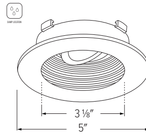
EKCL4723 - 4" ROUND BAFFLE
