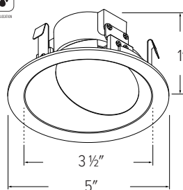
ELK4183 - 4" ROUND SLEEK WALL WASH REFLECTOR
