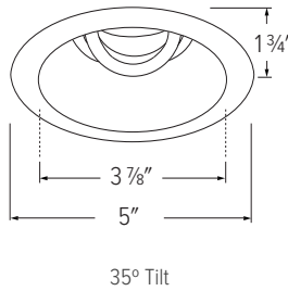
ELK4717 - 4" ROUND ADJUSTABLE DEEP REFLECTOR
