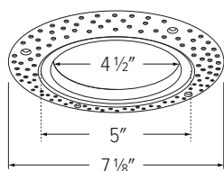
EL4FMR - 4" ROUND FLUSH MOUNT SPACKLE FRAME
