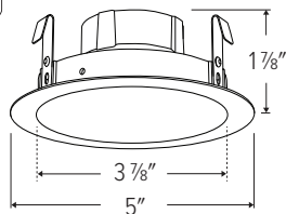
ELK4163 - 4" ROUND SLEEK REFLECTOR
