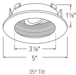
ELK4723 - 4" ROUND ADJUSTABLE BAFFLE
