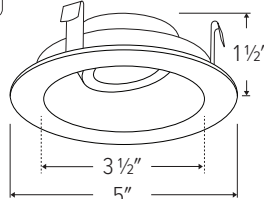
ELK4153 - 4" ROUND SLEEK REGRESSED EYEBALL
