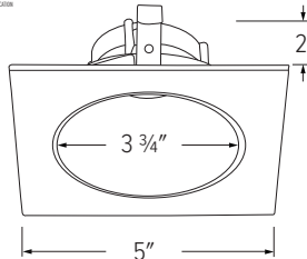
ELK4218 - 4" SQUARE DEEP REFLECTOR
