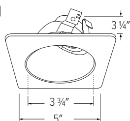
ELK4222 - 4" SQUARE ADJUSTABLE WALL WASH
