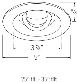
ELK4710 - 4" ROUND ADJUSTABLE REFLECTOR
