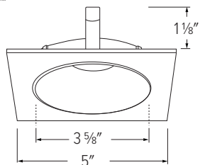
ELK4216 - 4" SQUARE SHALLOW REFLECTOR
