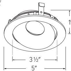
ELK4179 - 4" ROUND DIRECTIONAL GIMBAL
