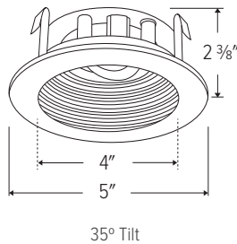
ELK4193 - 4" ROUND ADJUSTABLE BAFFLE
