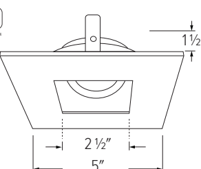
ELK4227 - 4" SQUARE ADJUSTABLE PINHOLE
