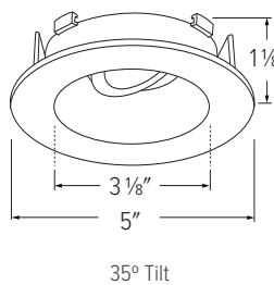
ELK4721 - 4" ROUND ADJUSTABLE REFLECTOR
