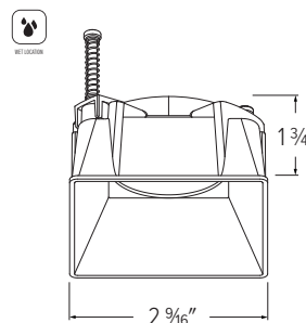
ELK370 - 3" SQUARE TRIMLESS REFLECTOR
