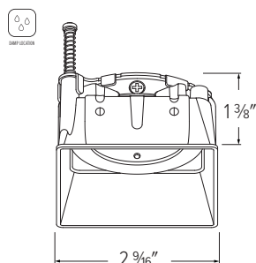
ELK381 - 3" SQUARE ADJUSTABLE TRIMLESS REFLECTOR
