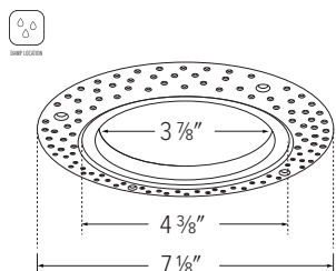
EL3FMR - 3" ROUND FLUSH MOUNT TRIM ADAPTER
