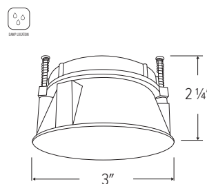
ELK315 - 3" ROUND ADJUSTABLE TRIMLESS REFLECTOR
