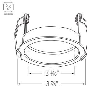
EL3WCRW - 3" ROUND KNIFE EDGE WOOD CEILING ADAPTOR
