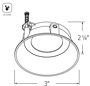
ELK308 - 3" ROUND TRIMLESS REFLECTOR
