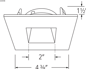
ELK3341 - 3" SQUARE REFLECTOR
