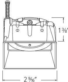
ELK381 - 3" SQUARE ADJUSTABLE TRIMLESS REFLECTOR
