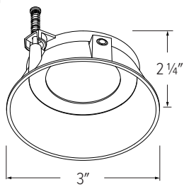
ELK308 - 3" ROUND TRIMLESS REFLECTOR
