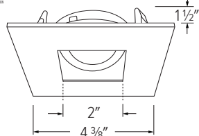
ELK3327 - 3" SQUARE ADJUSTABLE PINHOLE
