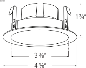
ELK3663 - 3" ROUND SLEEK REFLECTOR
