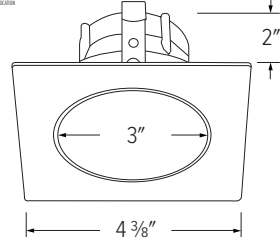
ELK3318 - 3" SQUARE DEEP REFLECTOR
