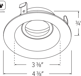
ELK3653 - 3" ROUND SLEEK REGRESSED EYEBALL
