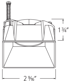
ELK370 - 3" SQUARE TRIMLESS REFLECTOR
