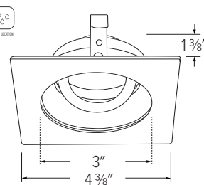
ELK3329 - 3" SQUARE ADJUSTABLE REFLECTOR
