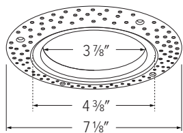
EL3FMR - 3" FLUSH MOUNT SPACKLE FRAME
