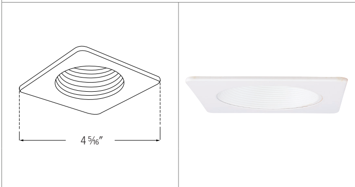
EL2393 - 3" SQUARE ON ROUND PHENOLIC BAFFLE
