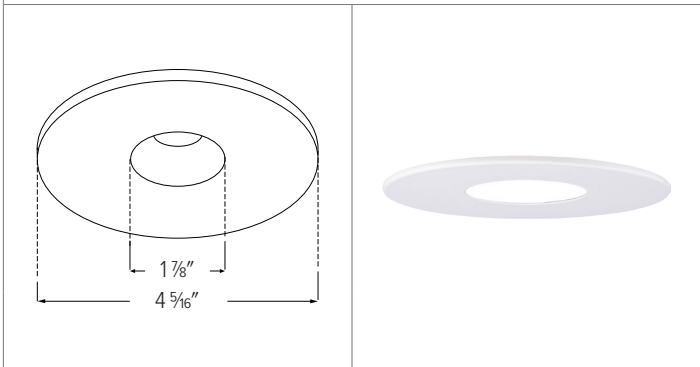
EL2619 - 3" DIE-CAST PINHOLE WITH REFLECTOR
