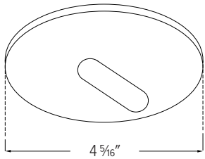
EL2620 - 3" DIE-CAST ADJUSTABLE SLOT APERTURE
