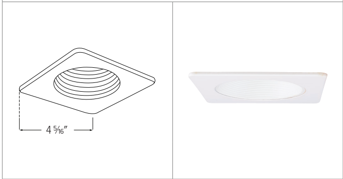
EL2393 - 3" SQUARE ON ROUND PHENOLIC BAFFLE TRIM
