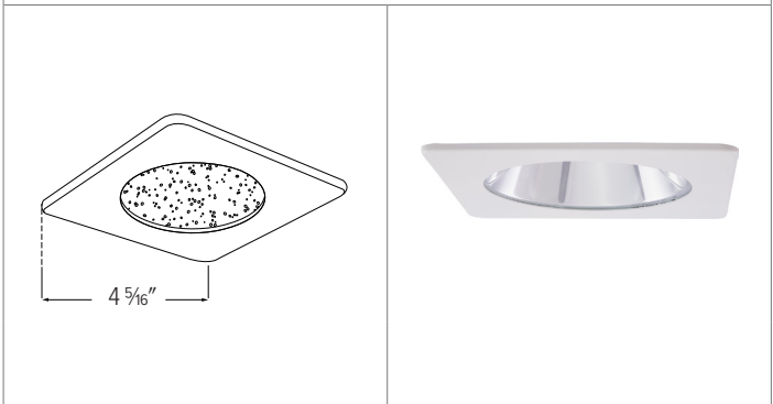
EL2313 - 3" DIE-CAST SQUARE LENSED SHOWER TRIMS
