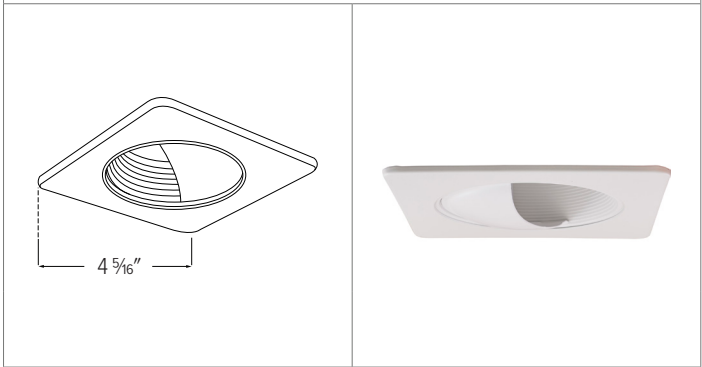
EL2395 - 3" DIE-CAST SQUARE WALL WASH BAFFLE TRIM
