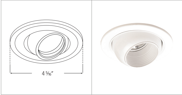
EL2698 - 3" DIE-CAST ADJUSTABLE EYEBALL TRIM
