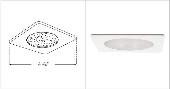
EL2312 - 3" DIE-CAST SQUARE LENSED SHOWER
