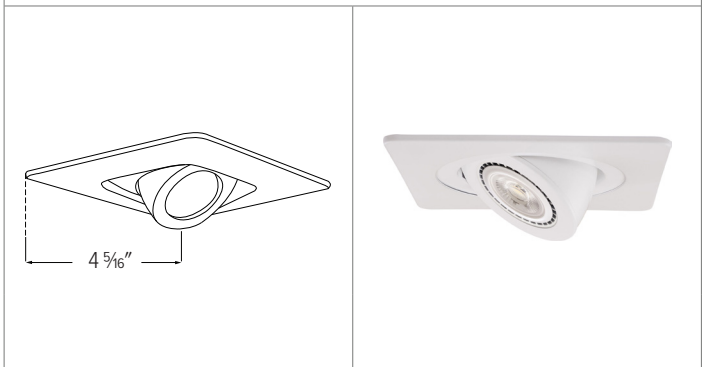
EL2388 - 3" DIE-CAST ADJUSTABLE SQUARE TRIM
