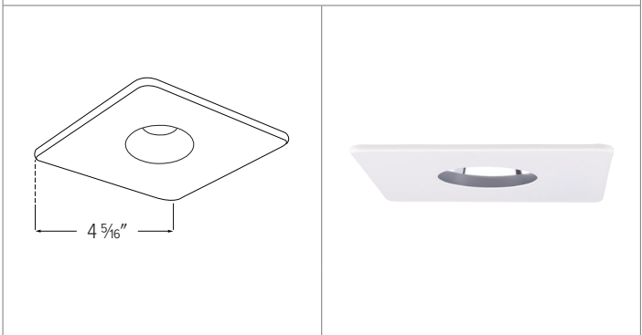
EL2319 - 3" SQUARE PINHOLE TRIM
