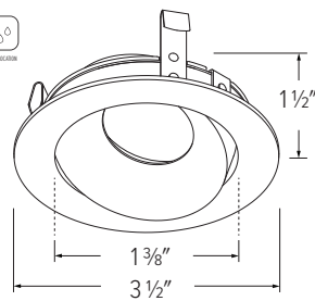
ELK3679 - 3" ROUND DIRECTIONAL GIMBAL
