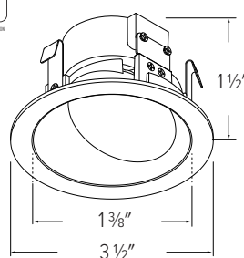
ELK3683 - 3" ROUND SLEEK WALL WASH REFLECTOR
