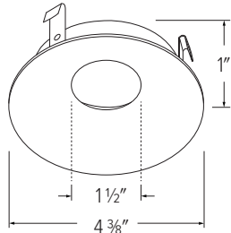
ELK3672 - 3" ROUND CURVED REFLECTOR
