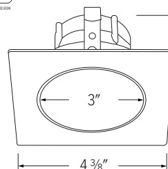
ELK3318 - 3" SQUARE DEEP REFLECTOR
