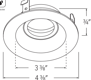
ELK3653 - 3" ROUND SLEEK REGRESSED EYEBALL
