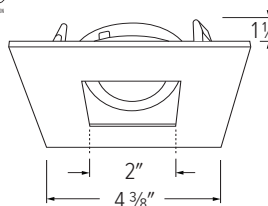
ELK3327 - 3" SQUARE ADJUSTABLE PINHOLE
