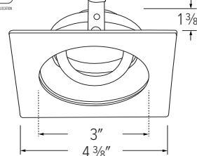
ELK3329 - 3" SQUARE ADJUSTABLE REFLECTOR
