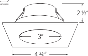
ELK3322 - 3" ADJUSTABLE REFLECTOR WALL WASH
