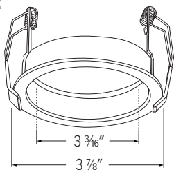
EL3WCRW - 3" ROUND KNIFE EDGE WOOD CEILING ADAPTOR
