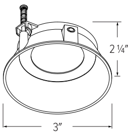
ELK308 - 3" ROUND TRIMLESS REFLECTOR
