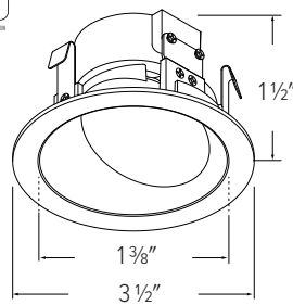
ELK3683 - 3" ROUND SLEEK LENSED WALL WASH REFLECTOR
