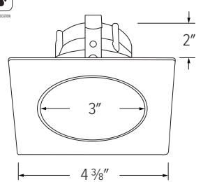
ELK3318 - 3" SQUARE DEEP REFLECTOR
