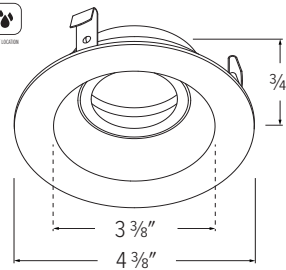
ELK3653 - 3" ROUND SLEEK REGRESSED EYEBALL
