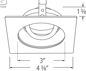
ELK3329 - 3" SQUARE ADJUSTABLE REFLECTOR
