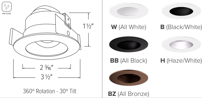
ELK2829 - 2" ROUND ADJUSTABLE REFLECTOR
