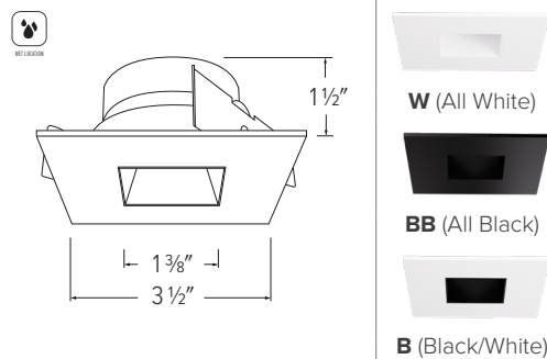
ELK2541 - 2" SQUARE REFLECTOR
