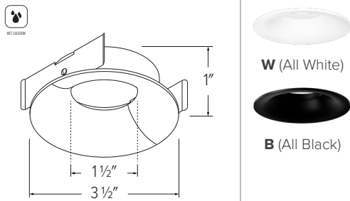
ELK2872 - 2" ROUND CURVED REFLECTOR
