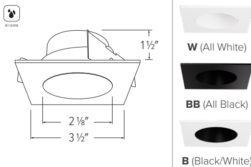
ELK2518 - 2" SQUARE DEEP REFLECTOR
