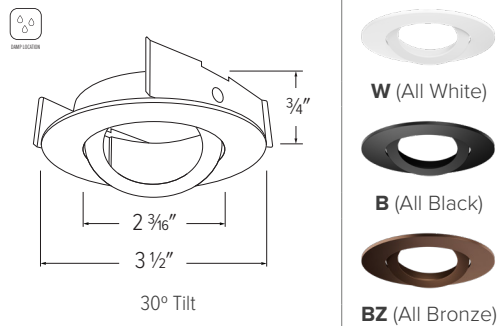
ELK2888 - 2" ROUND GIMBAL
