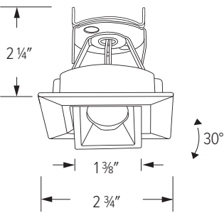
E1AK22 - 1" SQUARE PULL DOWN 30° ADJUSTABILITY
