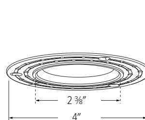
EL01SFR - 1" TRIMLESS SPACKLE FRAME
