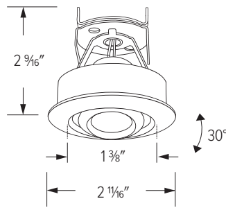
E1AK32 - 1" ROUND GIMBAL 30° ADJUSTABILITY
