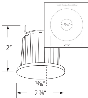
E1AK61 - 1" ROUND DOWNLIGHT
