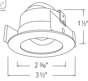
ELK2829 - 2" ROUND ADJUSTABLE REFLECTOR
