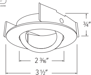
ELK2888 - 2" ROUND GIMBAL
