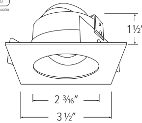
ELK2529 - 2" SQUARE ADJUSTABLE REFLECTOR
