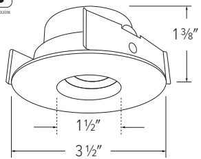
ELK2827 - 2" ROUND ADJUSTABLE PINHOLE
