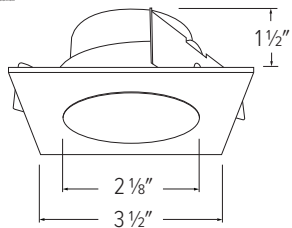
ELK2518 - 2" SQUARE DEEP REFLECTOR
