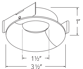
ELK2872 - 2" ROUND CURVED REFLECTOR
