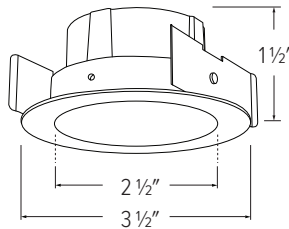
ELK2863 - 2" ROUND SLEEK REFLECTOR
