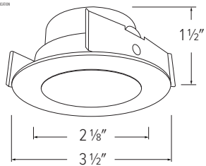
ELK2818 - 2" ROUND DEEP REFLECTOR
