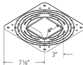
EL03SFS - 3" SQUARE TRIMLESS SPACKLE FRAME
