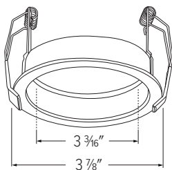
EL3WCRW - 3" ROUND KNIFE EDGE WOOD CEILING ADAPTOR
