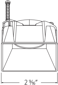
ELK370 - 3" SQUARE TRIMLESS REFLECTOR
