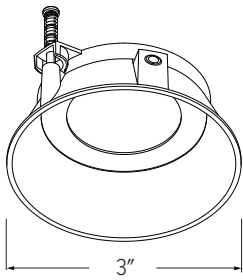
ELK308 - 3" ROUND TRIMLESS REFLECTOR
