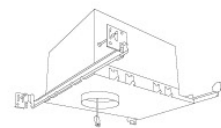
2" Maximum Adjustability ICA Housing 1500 lm (18.9W) w/ELK21 Series Module Not for use with ELK19 Series Module High Lumen New Construction
