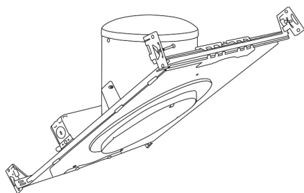
6" E26 Medium Base Sloped Housing New Construction
